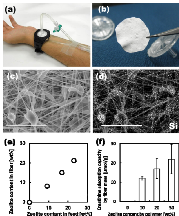
Fig. 1 a) Photographs of a wearable blood purification system, and b) a zeolite-polymer composite nanofiber mesh. c) SEM images of beta-type zeolite (10 wt%)/EVOH nanofiber composite (scale bar: 8 \mu\text{m} ), and d) EDX Si-mapping images. e) Relationship between zeolite contents in the fiber and their feed concentrations. f) Creatinine adsorption capacity of beta-type zeolite nanofibers by fiber mass.
